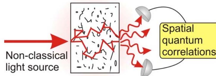
Fig 1. Illustration of multiple scattering process leading to spatial quantum correlations. A non-classical light source illuminates a medium consisting of a random distribution of scatterers. The incoming light is split into a multitude of different trajectories that perform a random walk through the medium. The number of photons exiting the medium in a specific direction can be anti-correlated with the number of photons in another direction, and this correlation depends on the quantum state of light illuminating the medium.
